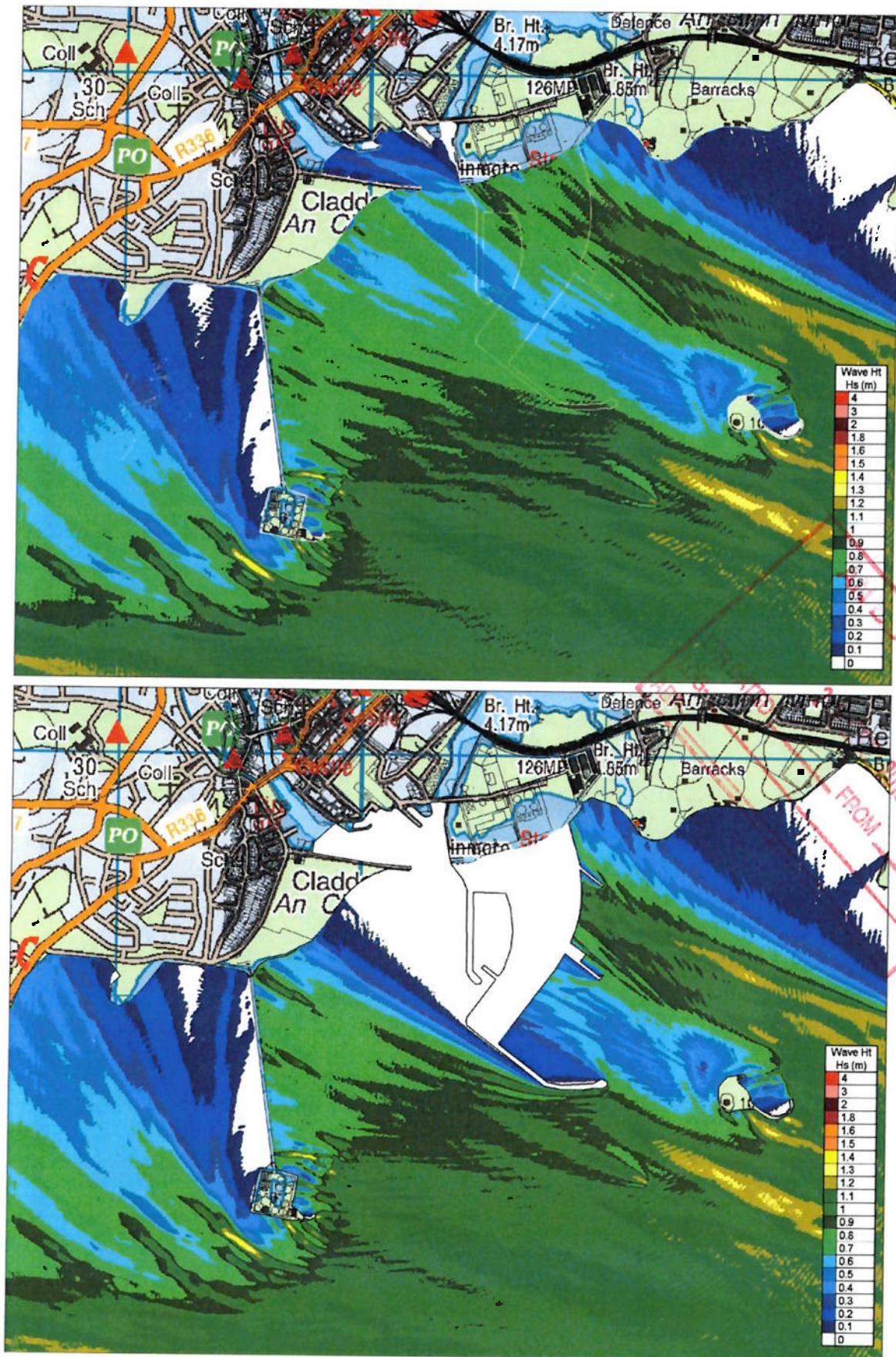
Figure 8.4.138 ARTEMIS Significant Wave Heights for local Design Storm Waves from the East-South-East for Existing and Proposed Case
