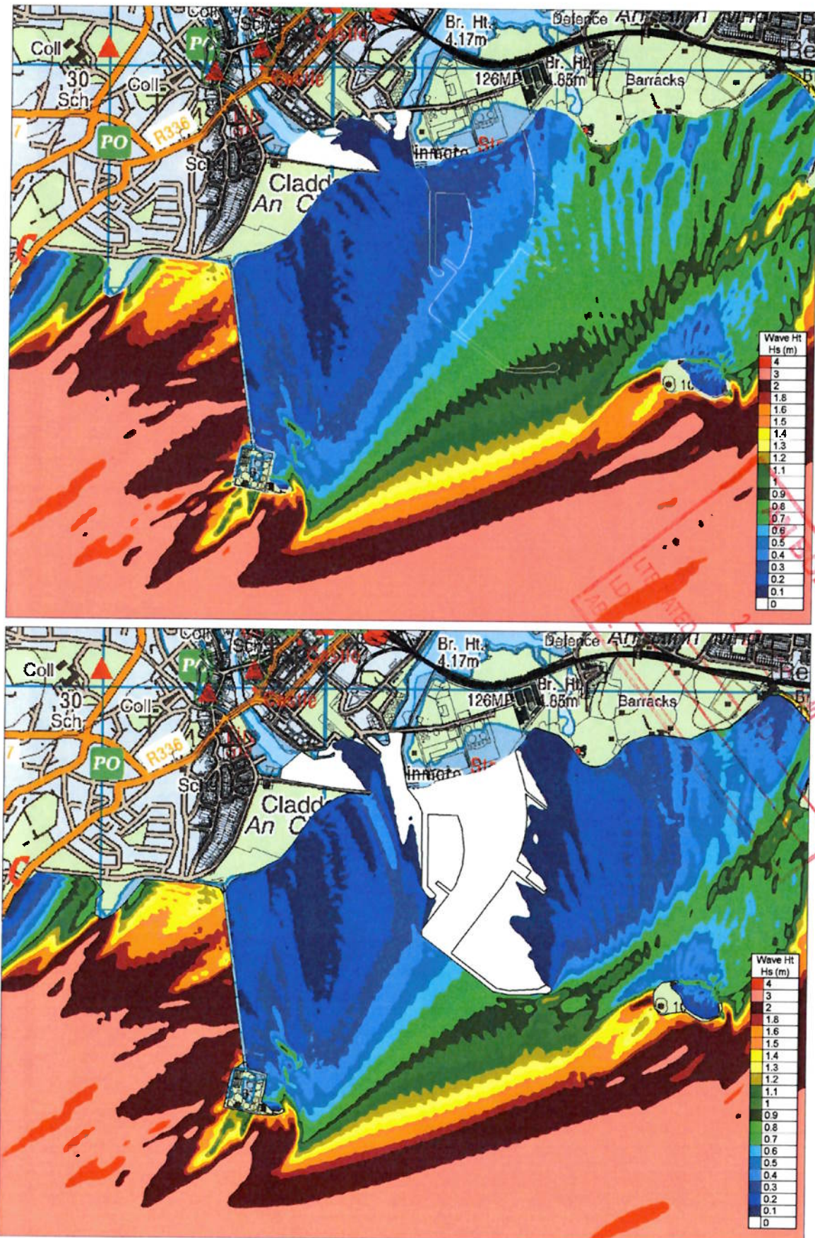
Figure 8.4.132 ARTEMIS Significant Wave Heights for Atlantic Storm from the West-South-West for Existing and Proposed Case
