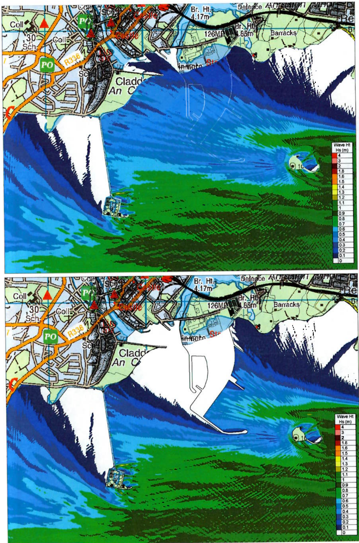
Figure 8.4.139 ARTEMIS Significant Wave Heights for local Design Storm Waves from the East for Existing and Proposed Case
