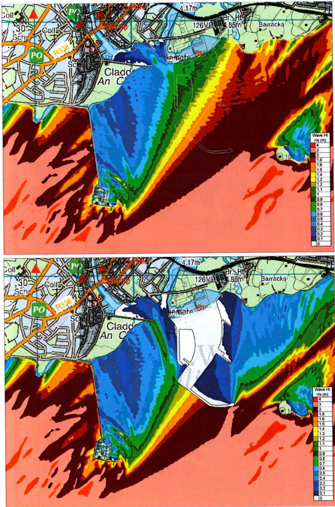
Figure 8.4.133 ARTEMIS Significant Wave Heights for Atlantic Storm from the South-West for Existing and Proposed Case
