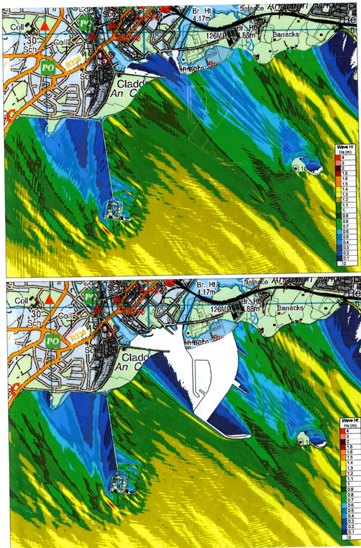
Figure 8.4.137 ARTEMIS Significant Wave Heights for local Design Storm Waves from the South-East for Existing and Proposed Case
