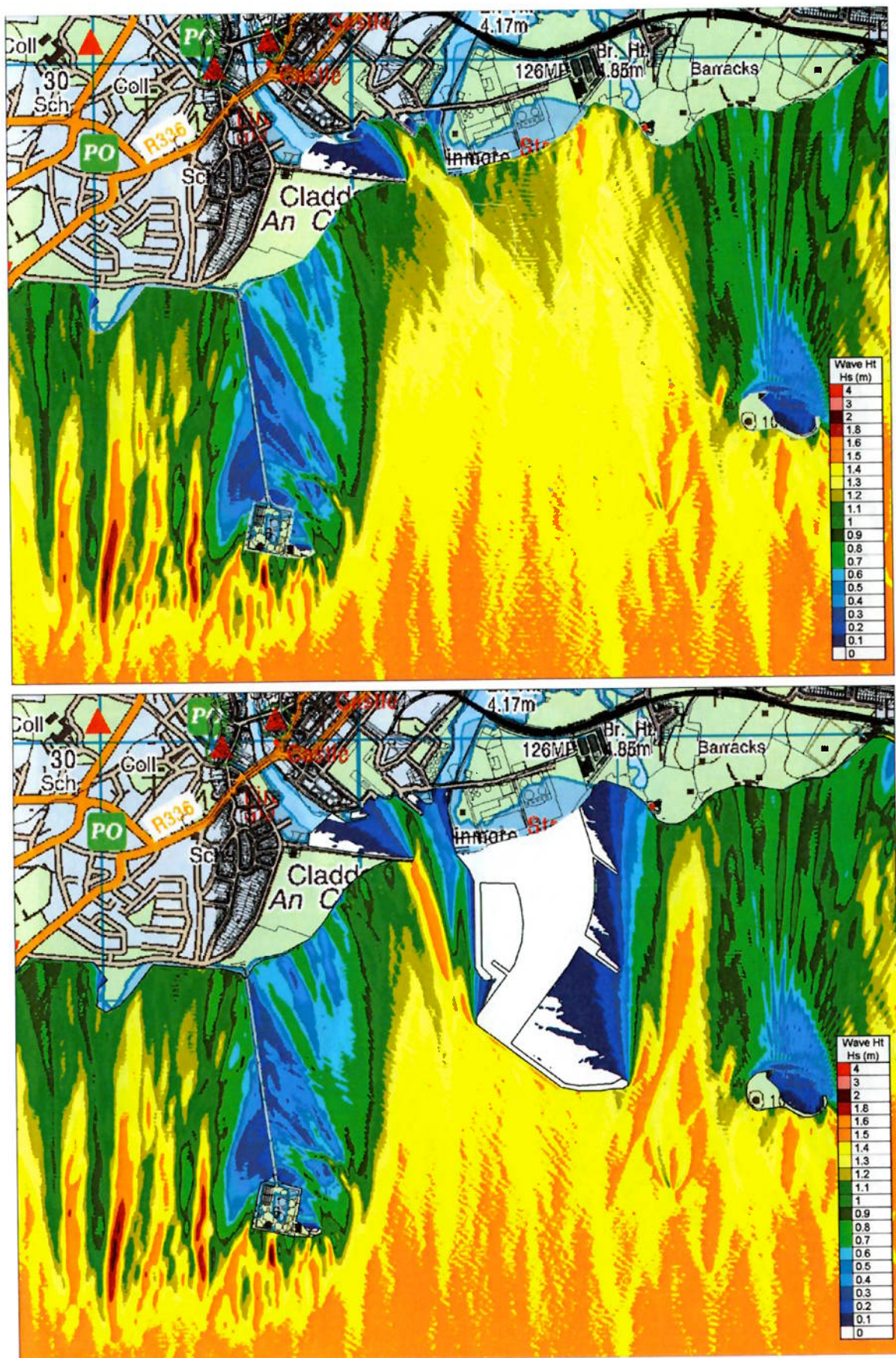
Figure 8.4.135 ARTEMIS Significant Wave Heights for local Design Storm Waves from the South for Existing and Proposed Case
