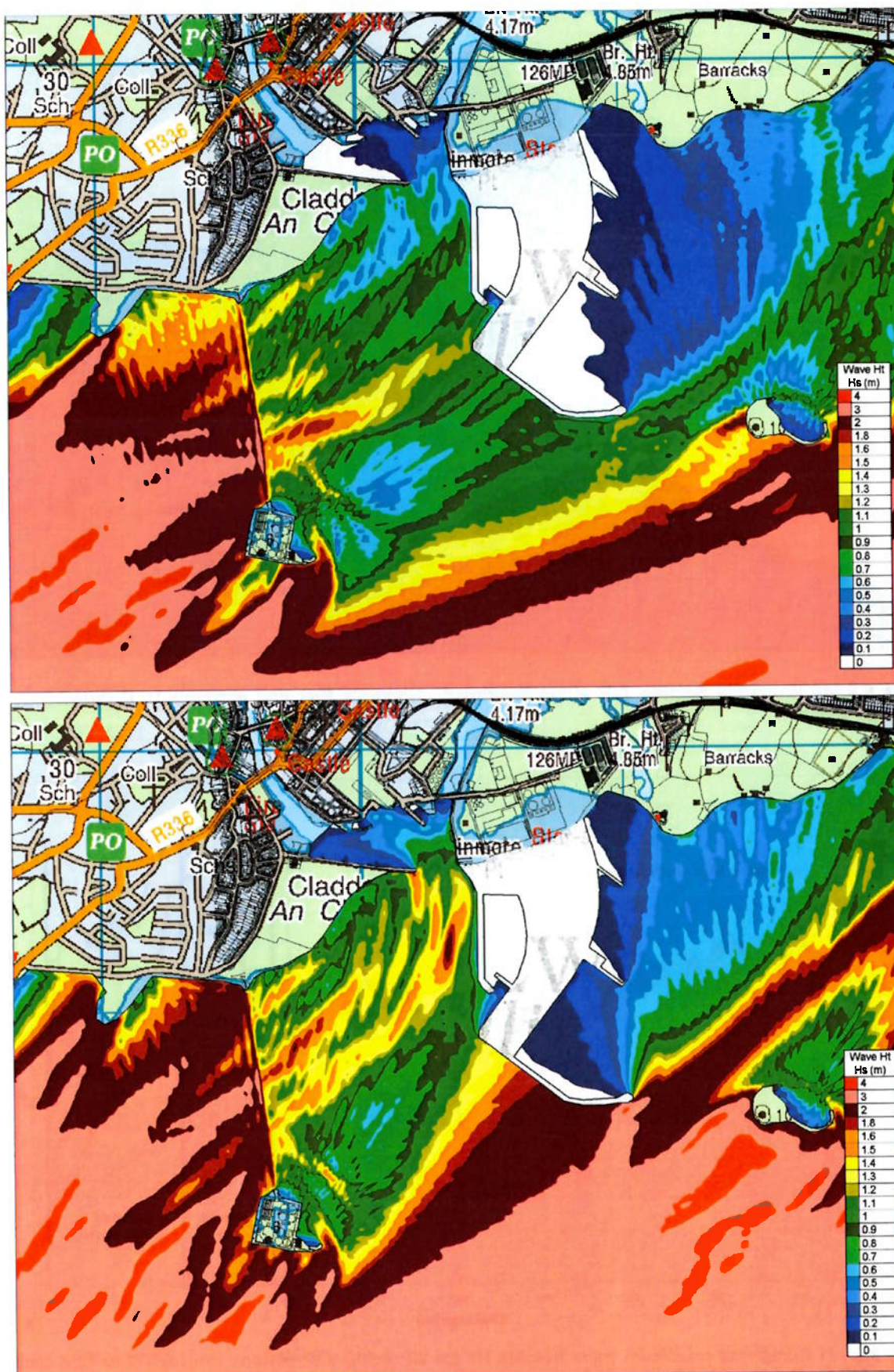
Figure 8.4.142 West-South-West Design Wave at extreme highwater of 4.635 m O.D. Malin to examine the ability of Mutton Island Causeway to protect the Harbour and Marina area from West-South-West and south-west deepwater design waves
