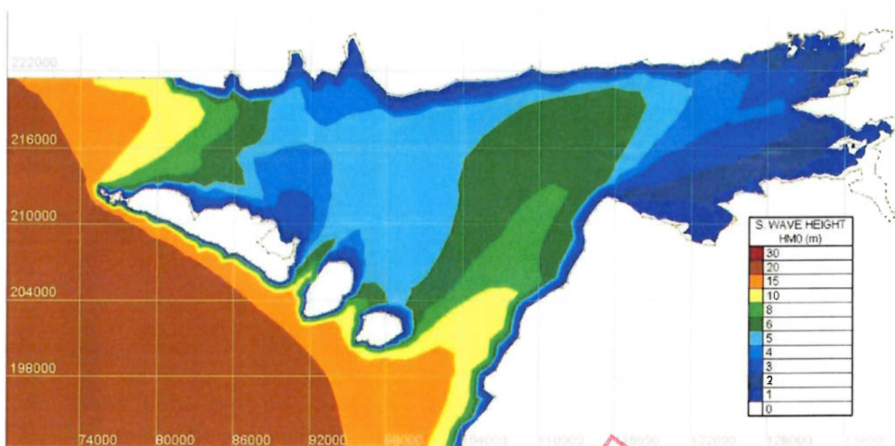
Figure 8.4.129 Wave climate under 50-year southwest wind conditions
